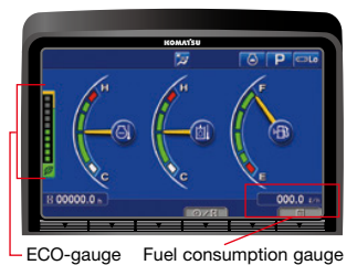
ECO-gauge Fuel consumption gauge
